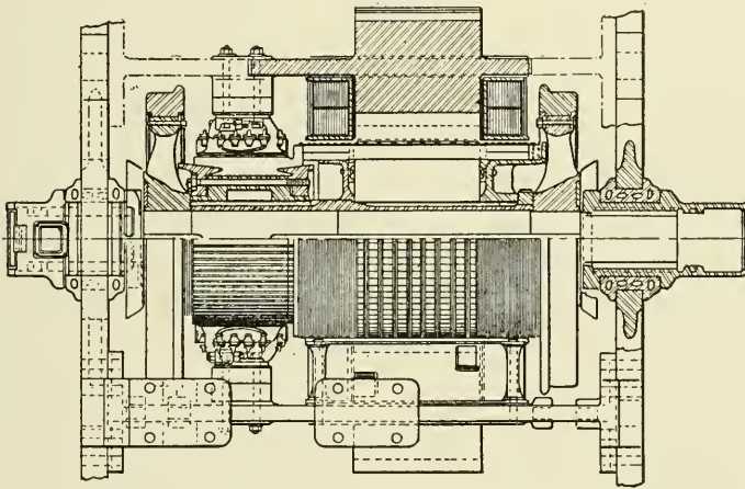
Fig. 247. Section of Motor Used on Locomotive Shown in Fig. 246
